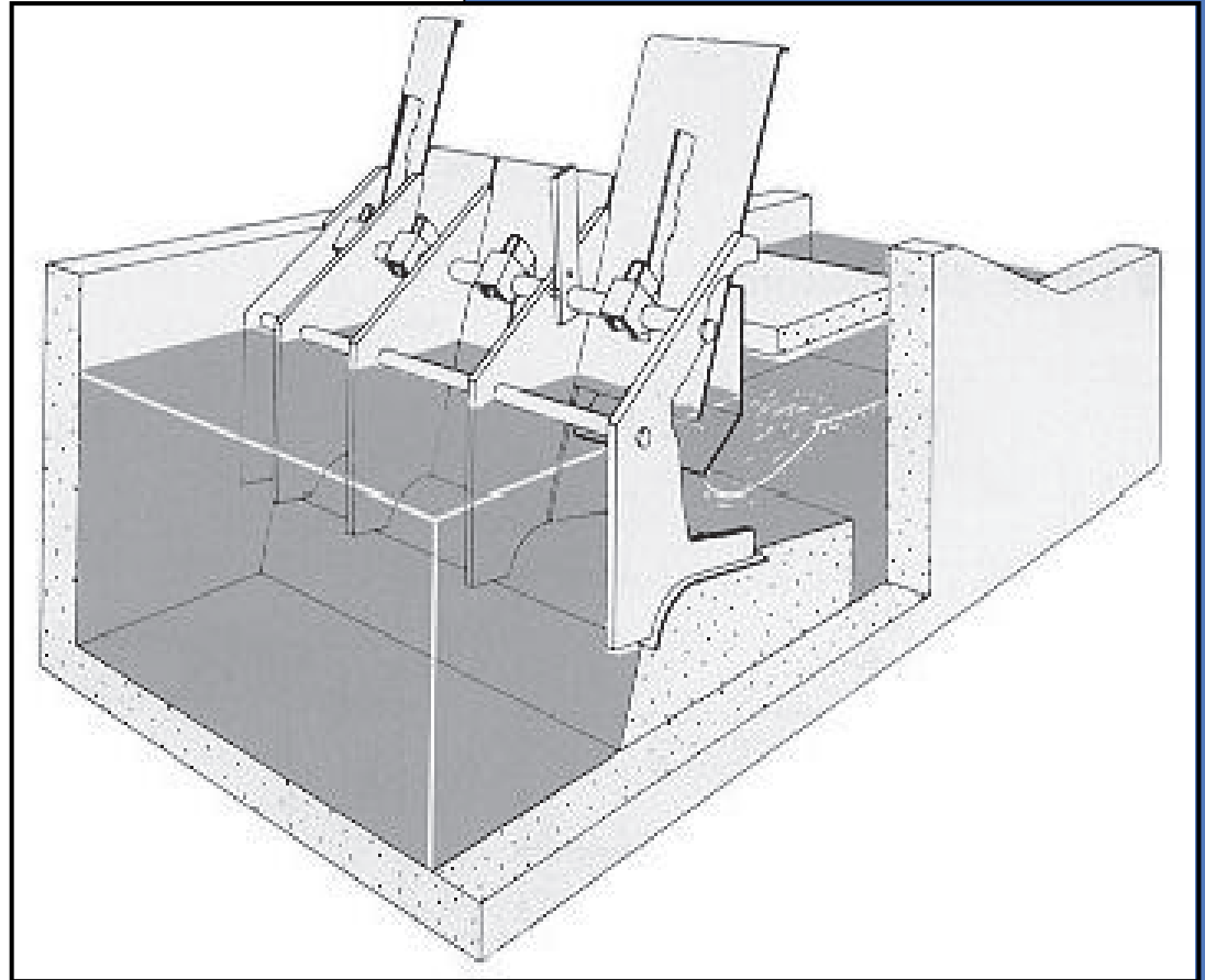
Battery of distributors DL, 1700 l/s (one 1000 l/s unit + one 700 l/s unit).
